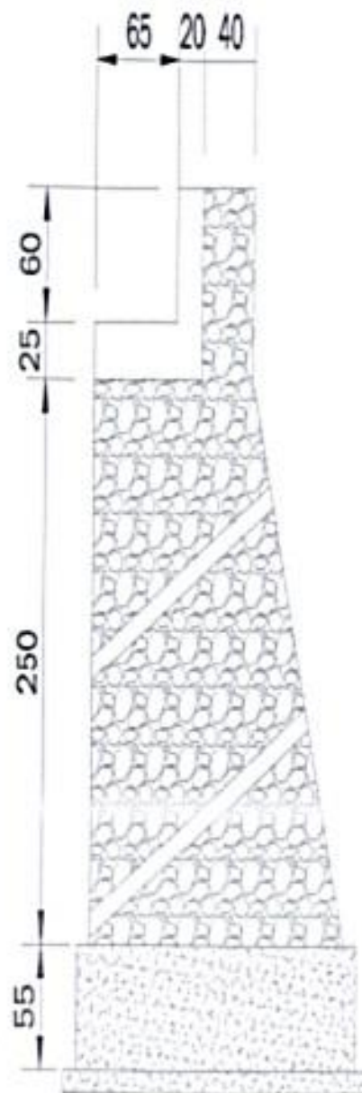
ABUTMENT
